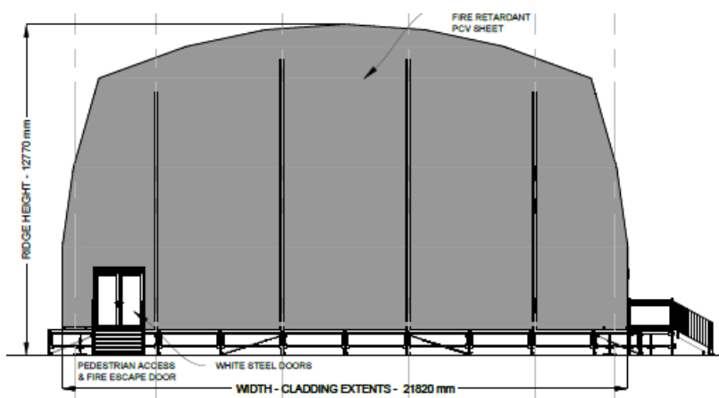
Workshop 6 Elevation
